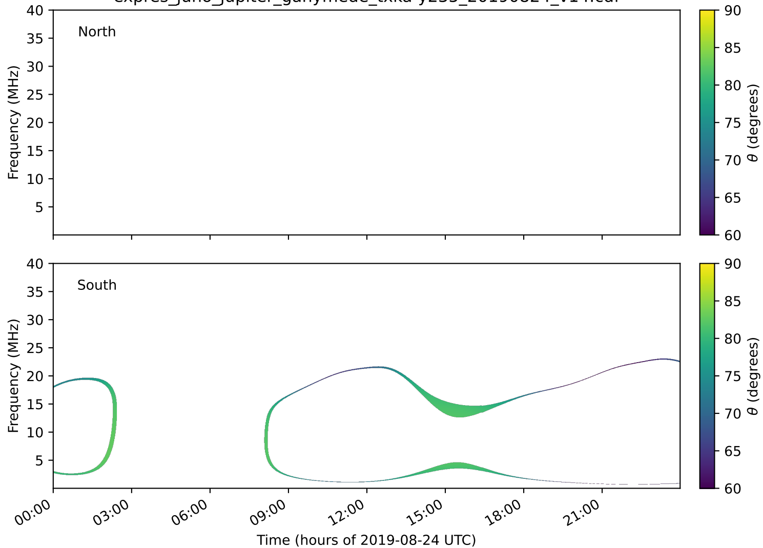
expres_juno_jupiter_ganymede_txka-y235_20190824_v14.cdf
