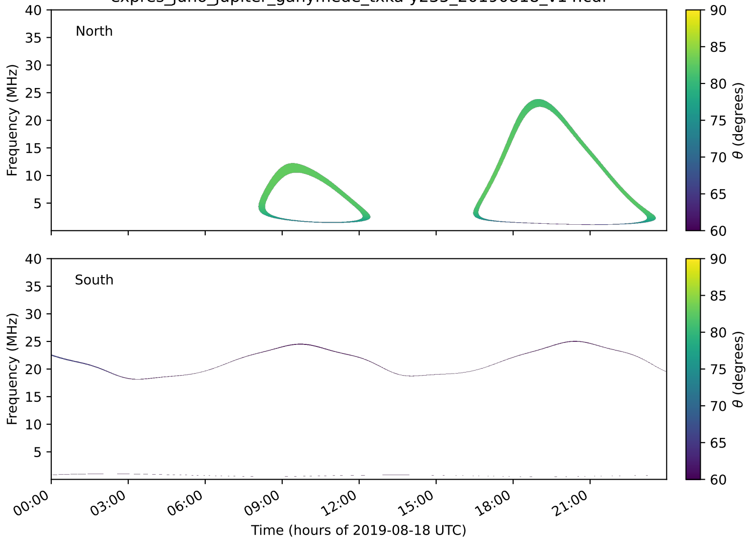
expres_juno_jupiter_ganymede_txka-y235_20190818_v14.cdf
