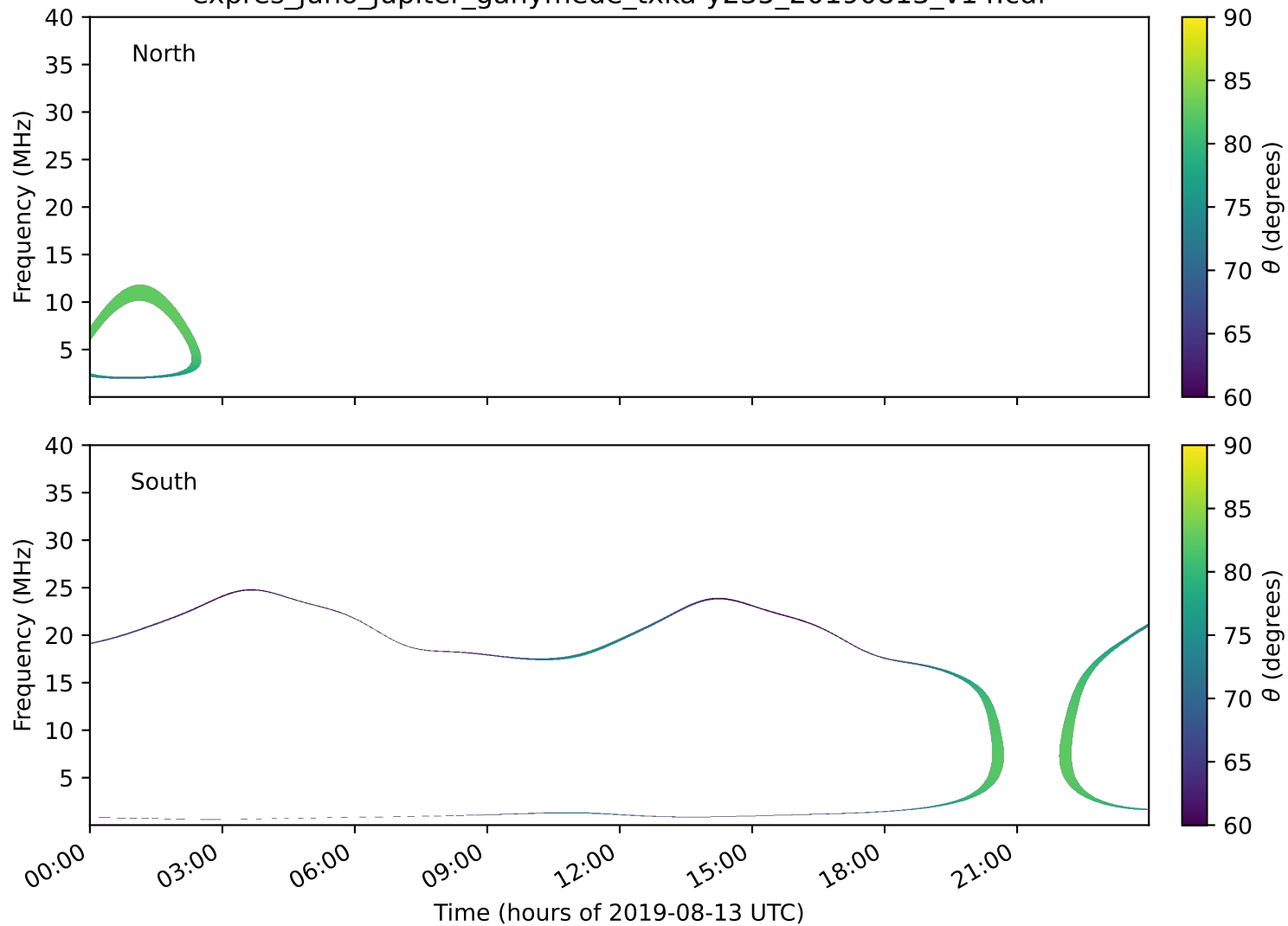
expres_juno_jupiter_ganymede_txka-y235_20190813_v14.cdf
