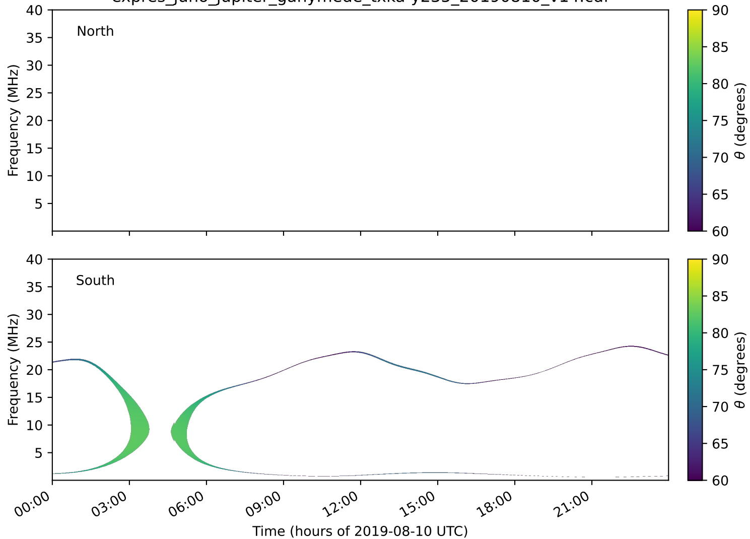
expres_juno_jupiter_ganymede_txka-y235_20190810_v14.cdf
