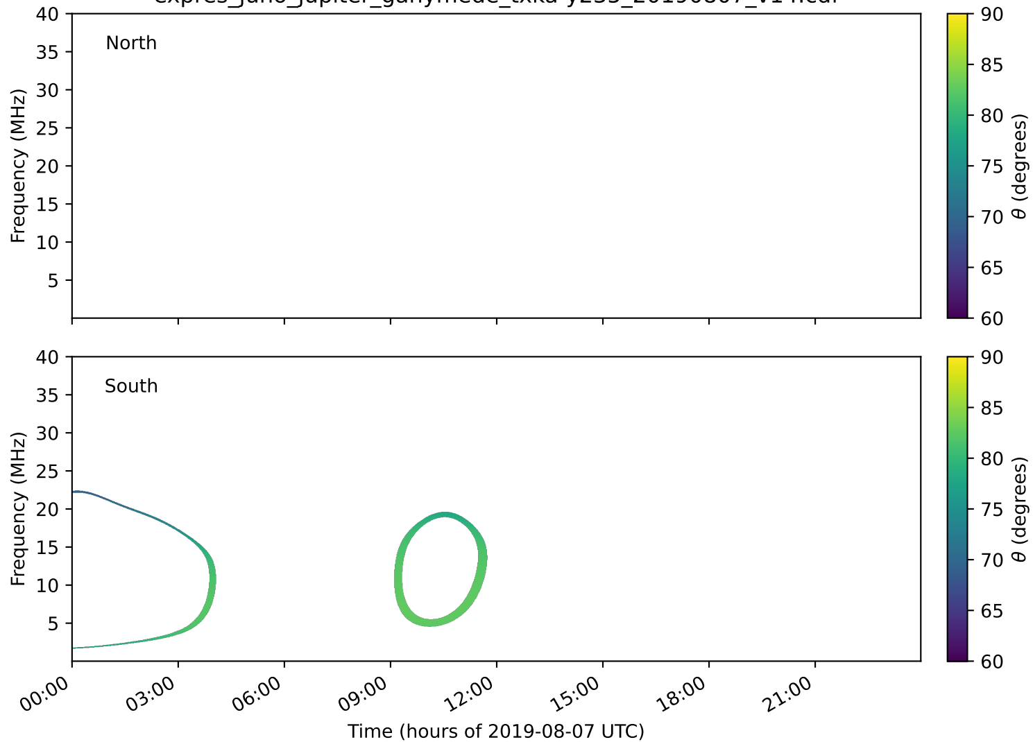
expres_juno_jupiter_ganymede_txka-y235_20190807_v14.cdf
