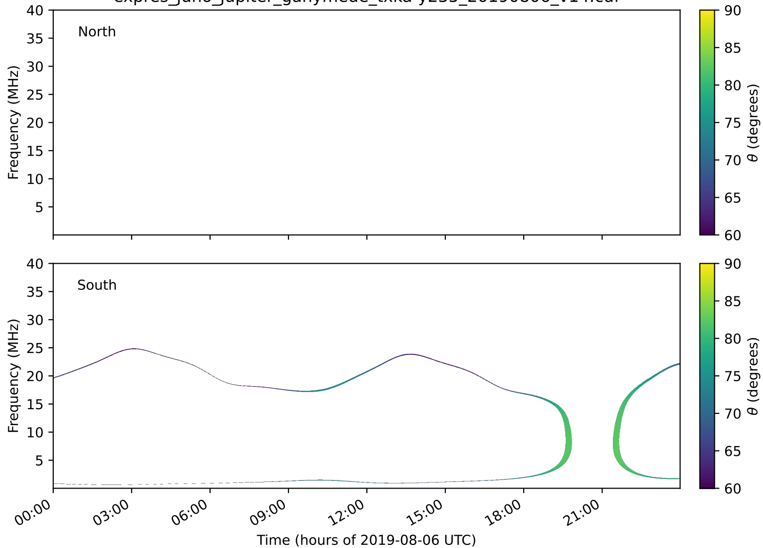
expres_juno_jupiter_ganymede_txka-y235_20190806_v14.cdf
