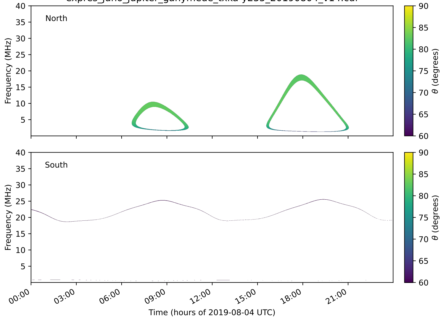
expres_juno_jupiter_ganymede_txka-y235_20190804_v14.cdf
