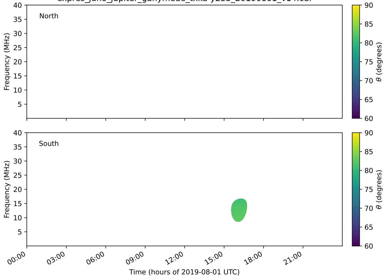
expres_juno_jupiter_ganymede_txka-y235_20190801_v14.cdf
