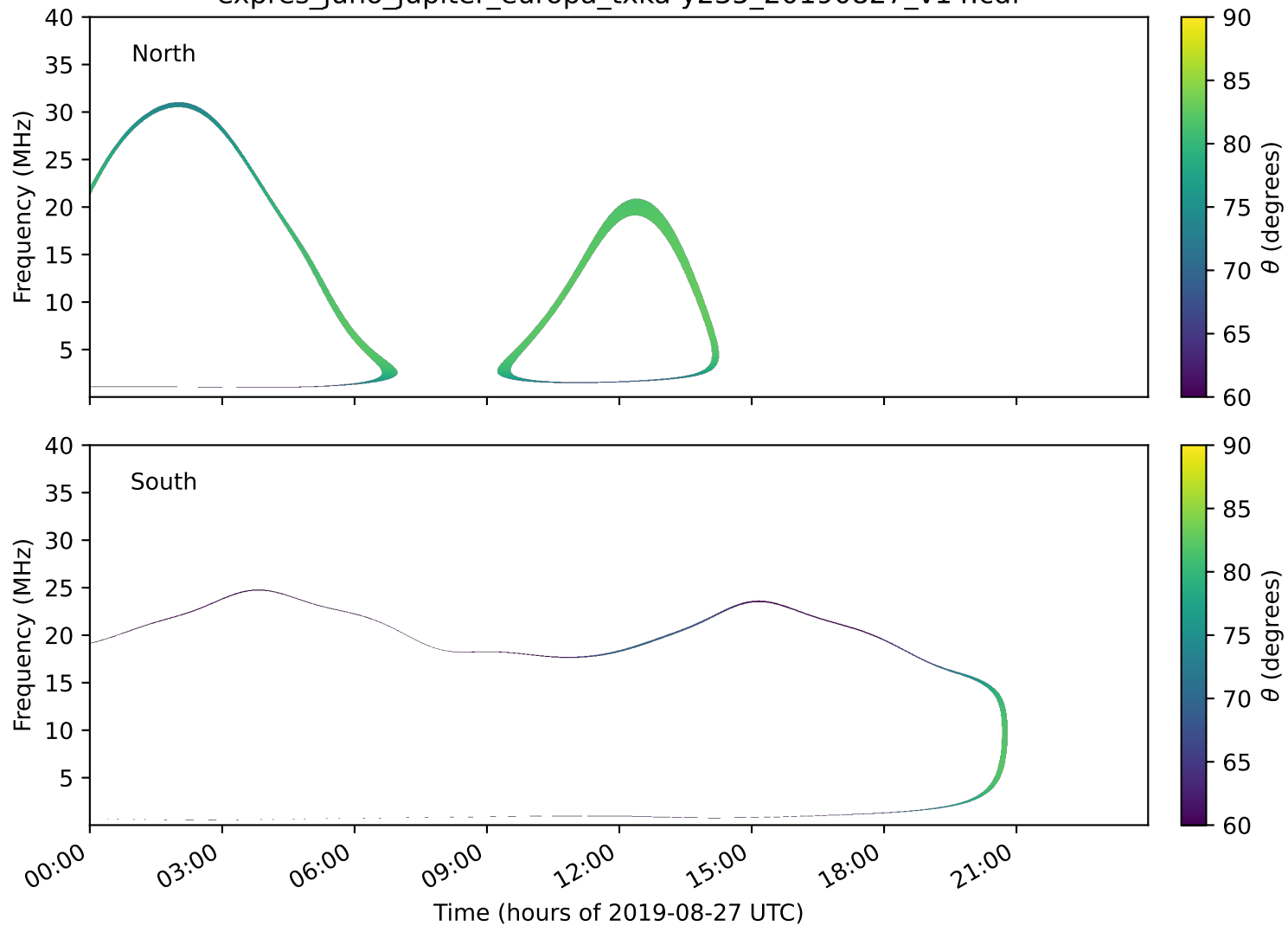
expres_juno_jupiter_europa_txka-y235_20190827_v14.cdf
