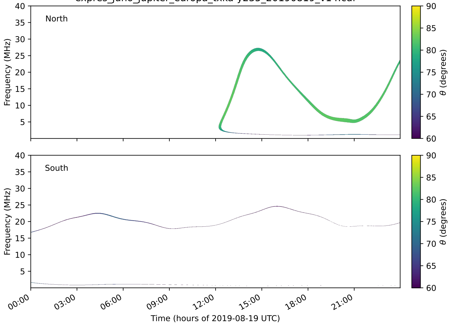
expres_juno_jupiter_europa_txka-y235_20190819_v14.cdf
