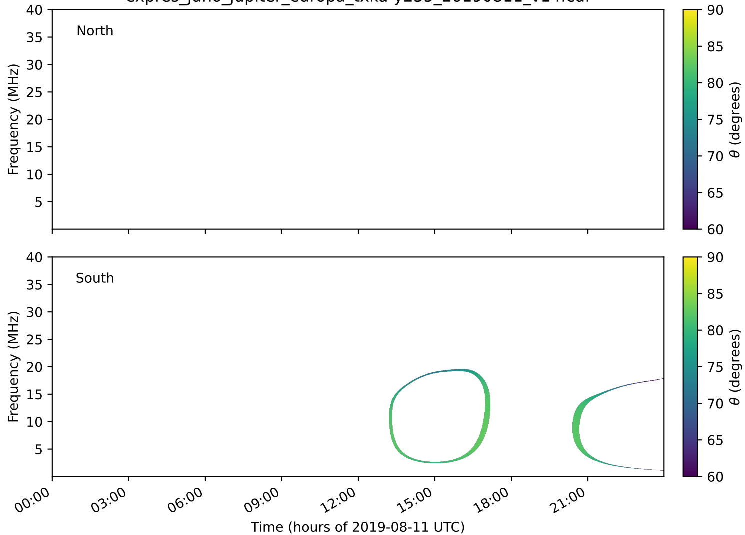
expres_juno_jupiter_europa_txka-y235_20190811_v14.cdf
