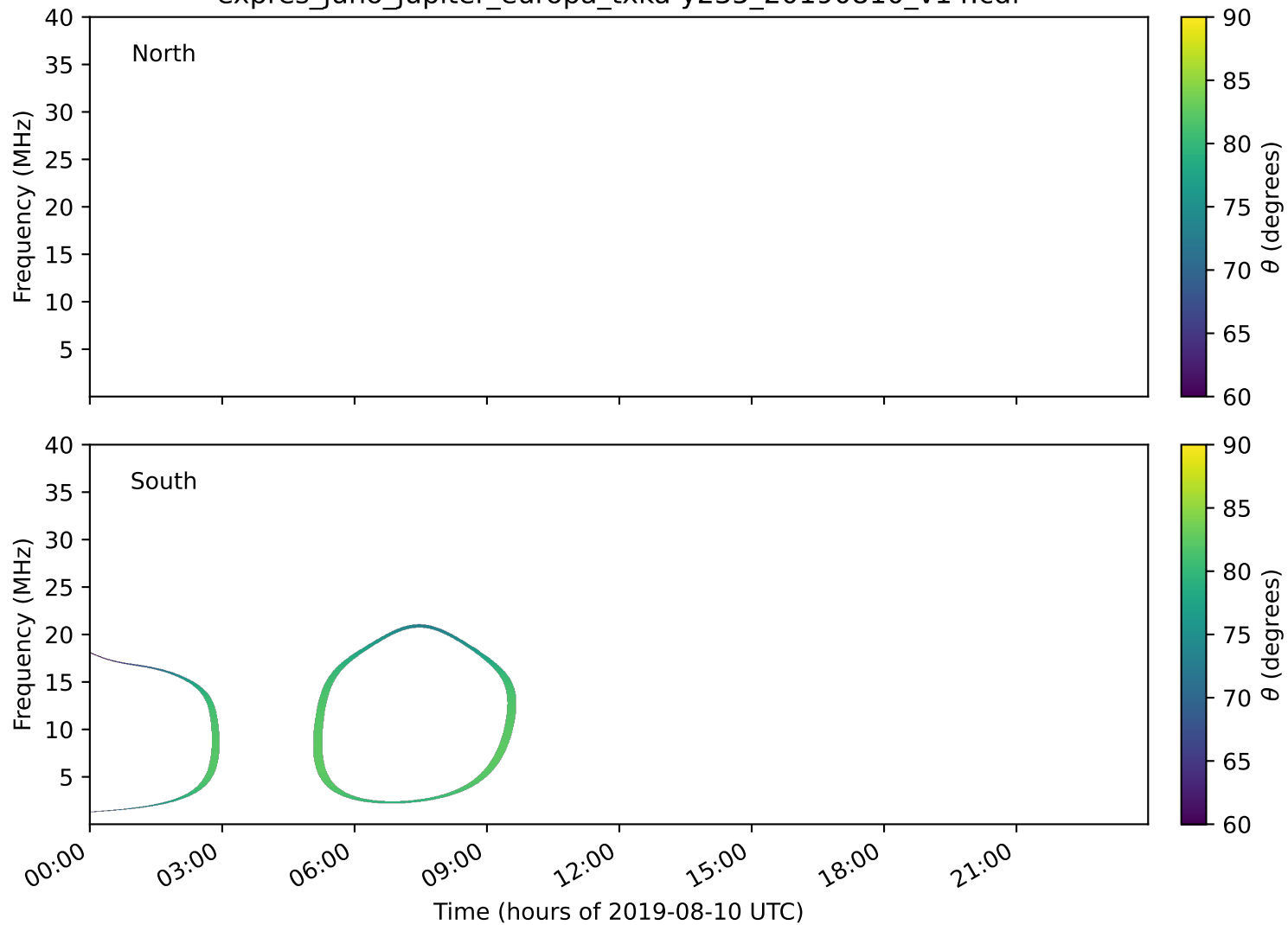
expres_juno_jupiter_europa_txka-y235_20190810_v14.cdf
