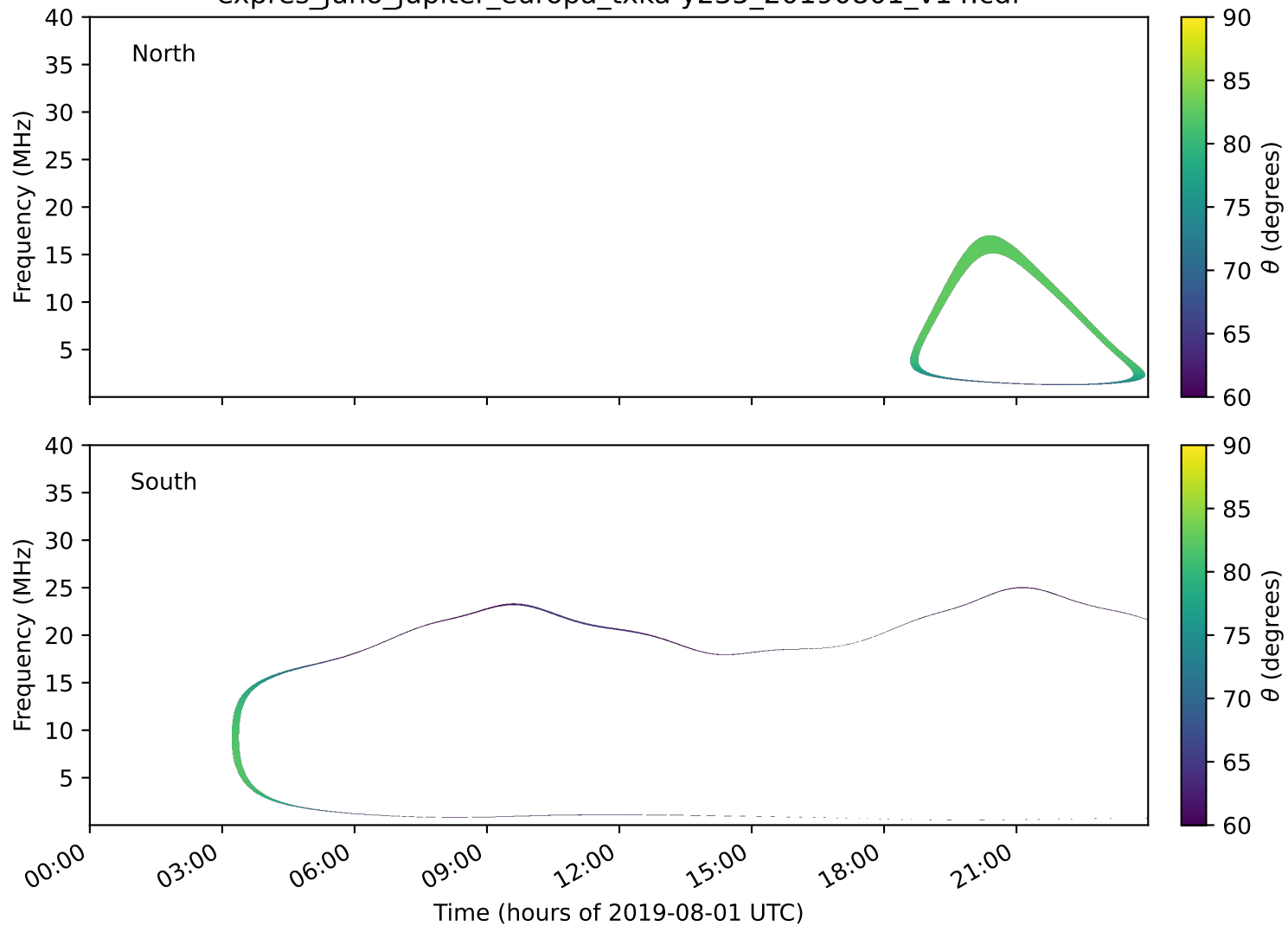
expres_juno_jupiter_europa_txka-y235_20190801_v14.cdf
