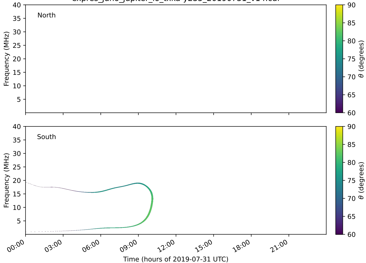
expres_juno_jupiter_io_txka-y235_20190731_v14.cdf
