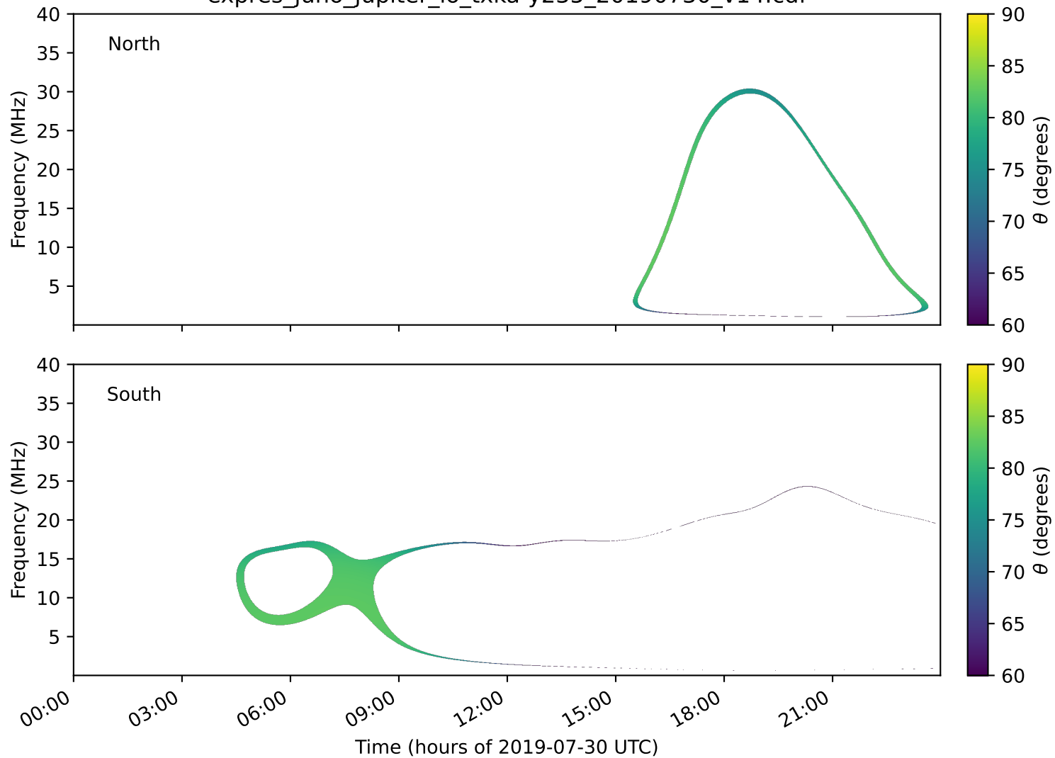
expres_juno_jupiter_io_txka-y235_20190730_v14.cdf
