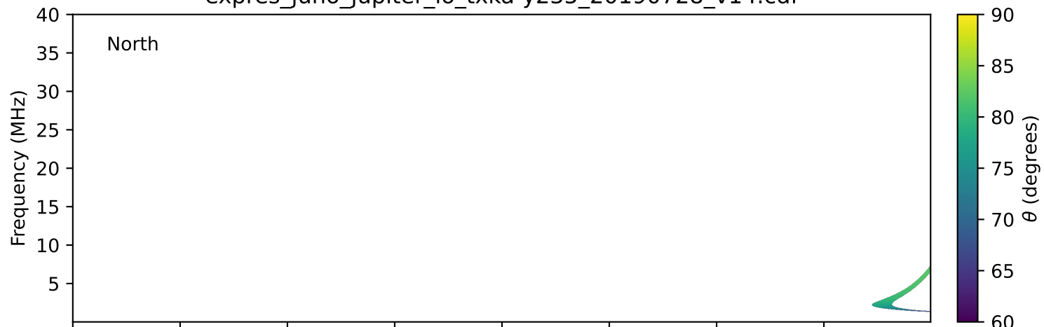
expres_juno_jupiter_io_txka-y235_20190728_v14.cdf
