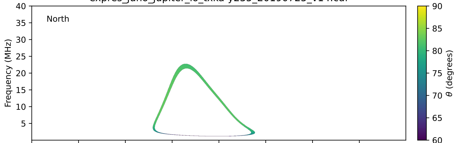
expres_juno_jupiter_io_txka-y235_20190725_v14.cdf
