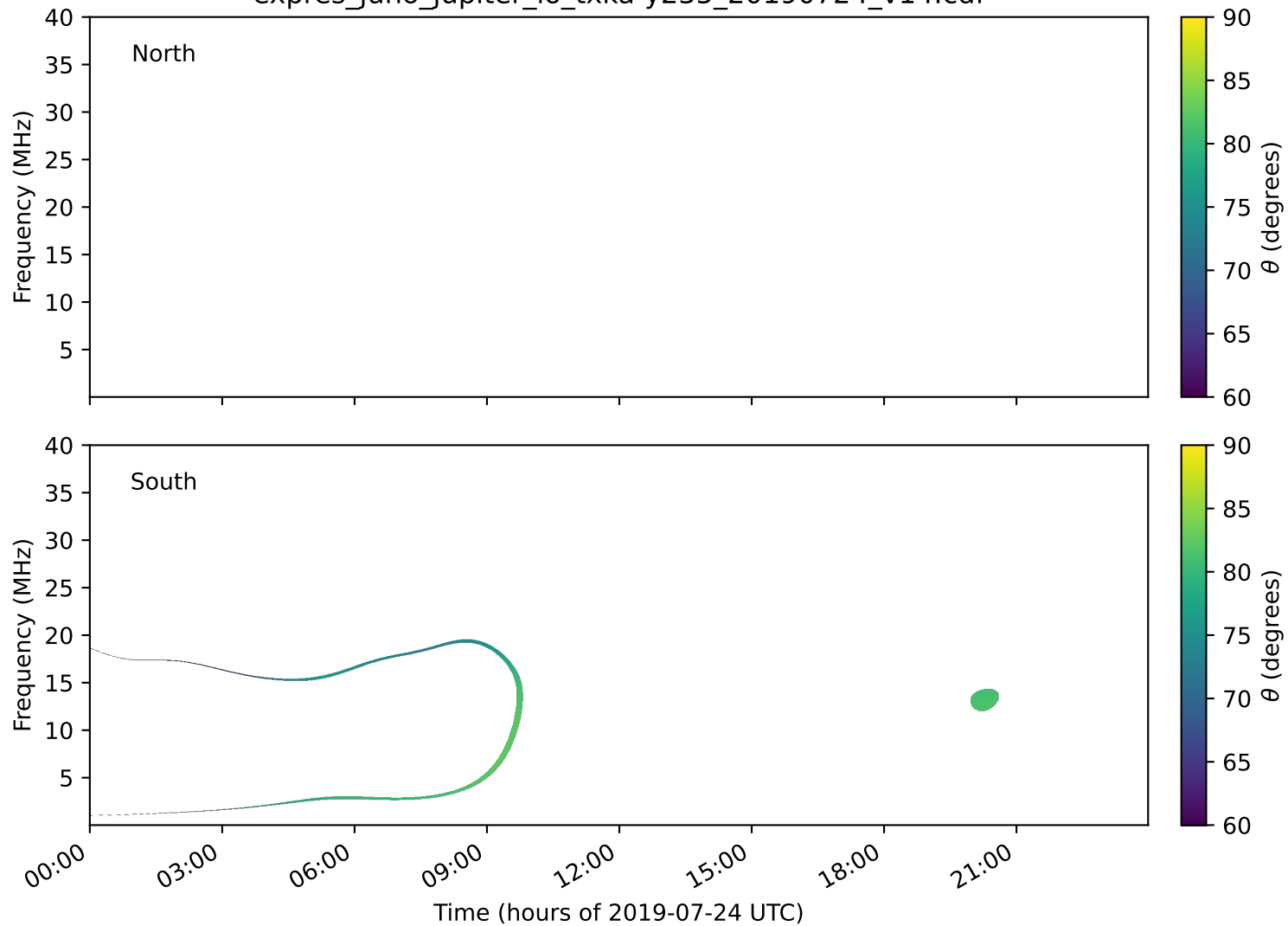
expres_juno_jupiter_io_txka-y235_20190724_v14.cdf
