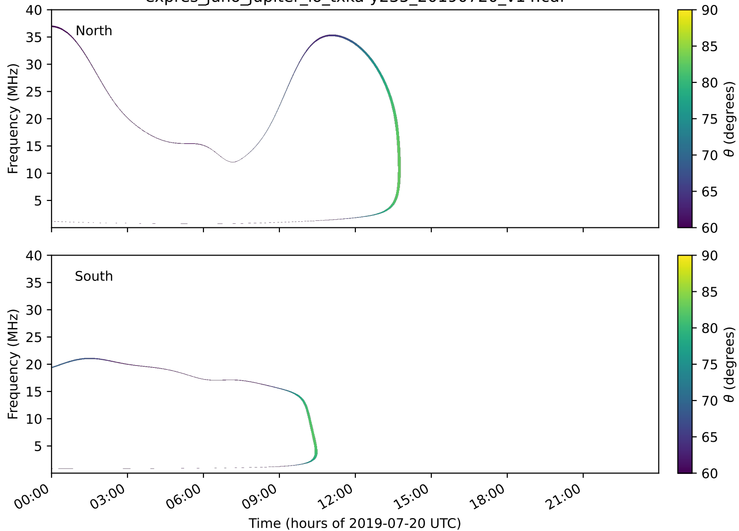
expres_juno_jupiter_io_txka-y235_20190720_v14.cdf
