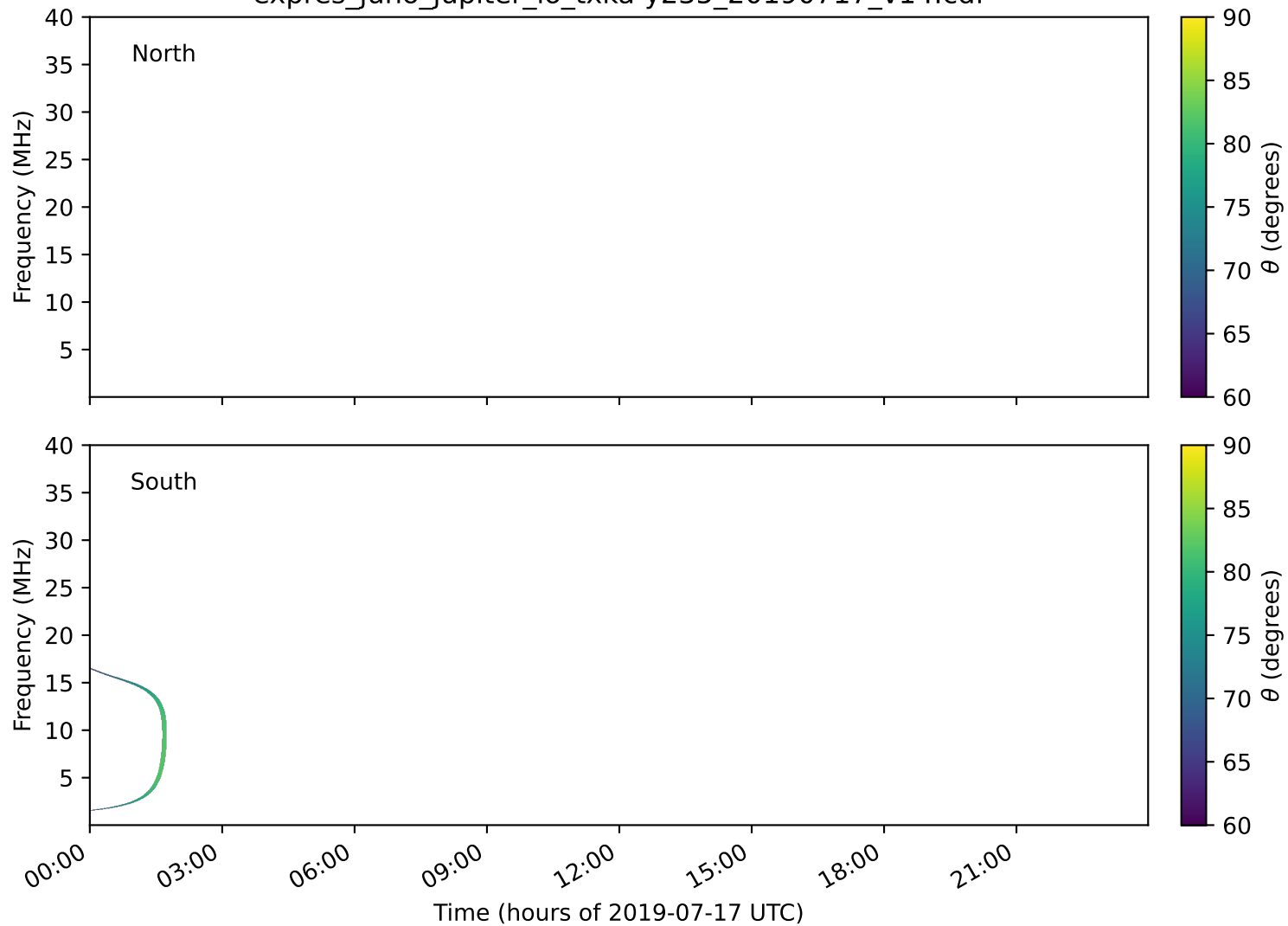
expres_juno_jupiter_io_txka-y235_20190717_v14.cdf
