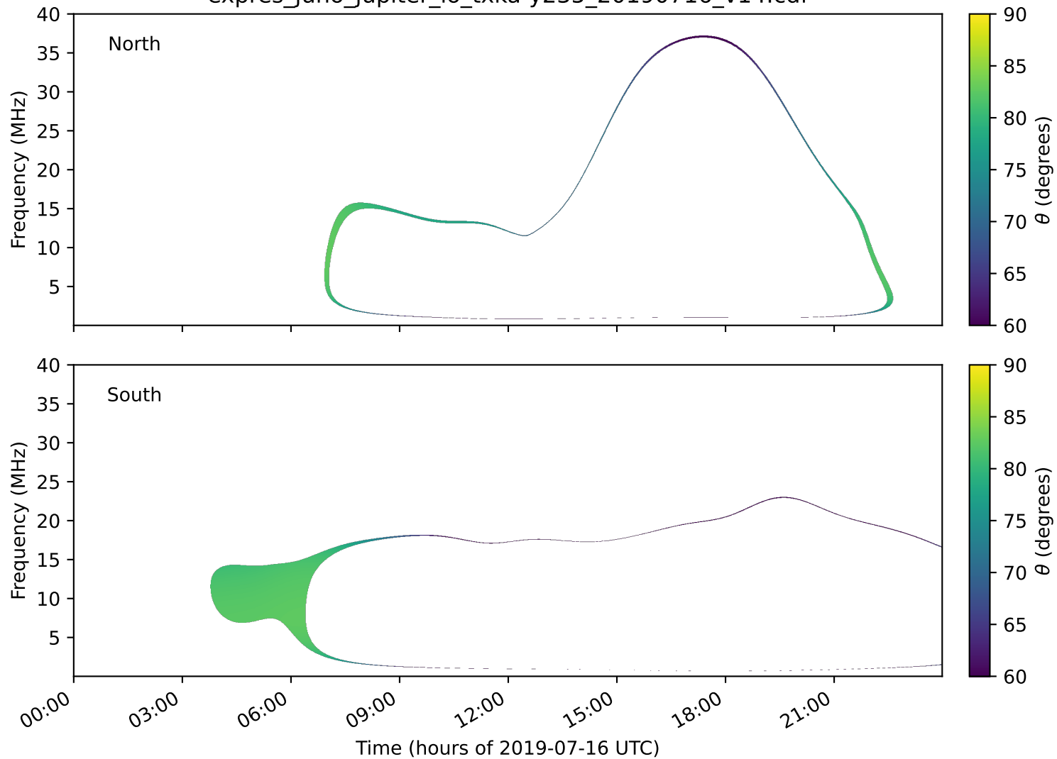
expres_juno_jupiter_io_txka-y235_20190716_v14.cdf
