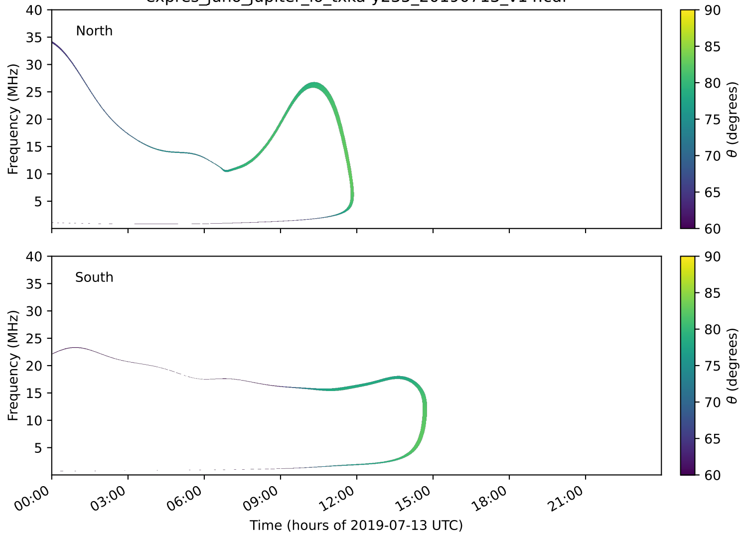
expres_juno_jupiter_io_txka-y235_20190713_v14.cdf
