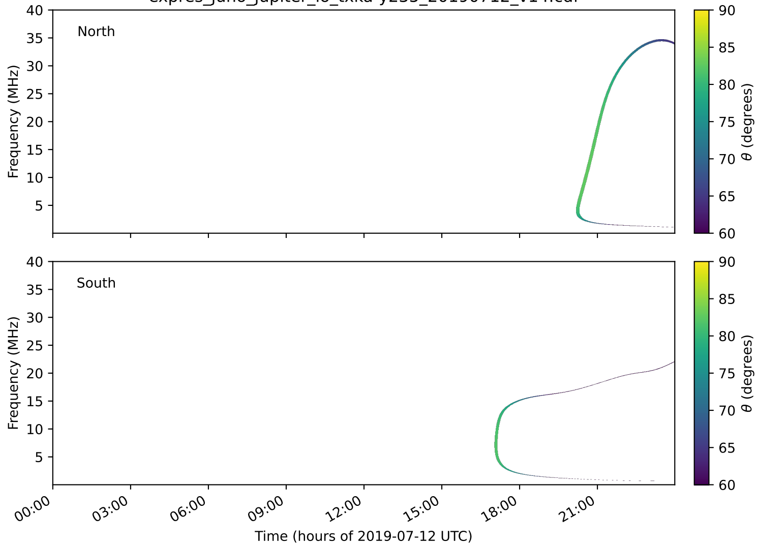
expres_juno_jupiter_io_txka-y235_20190712_v14.cdf
