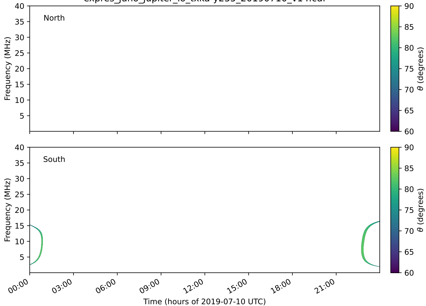
expres_juno_jupiter_io_txka-y235_20190710_v14.cdf
