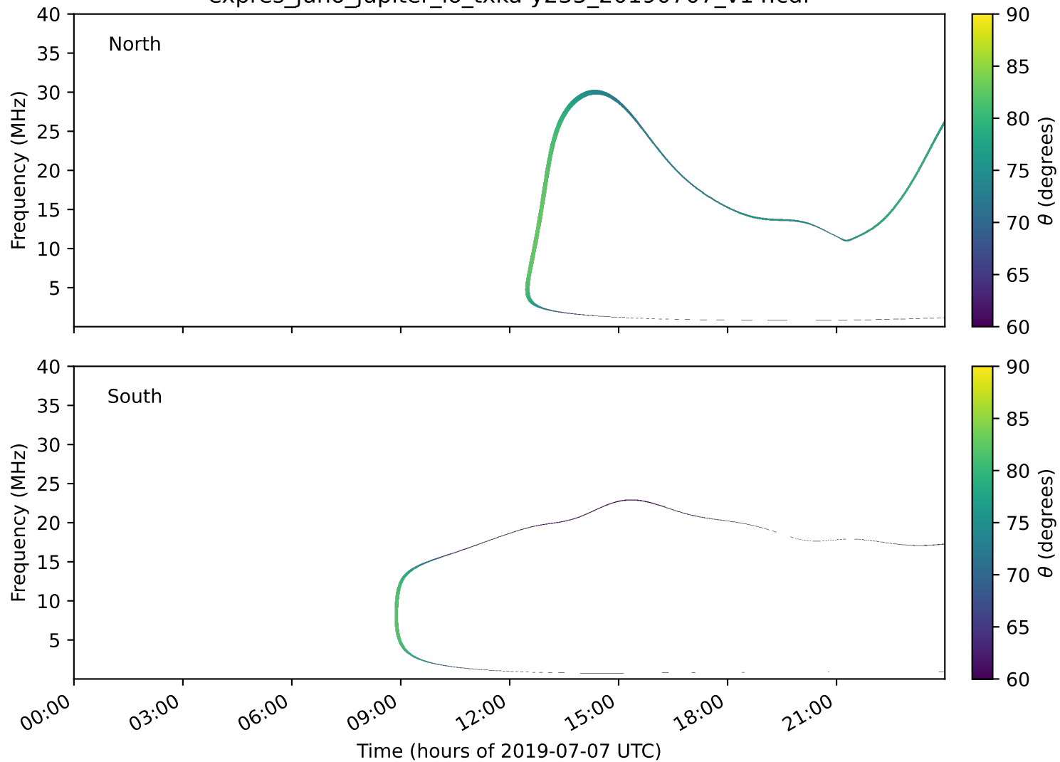
expres_juno_jupiter_io_txka-y235_20190707_v14.cdf
