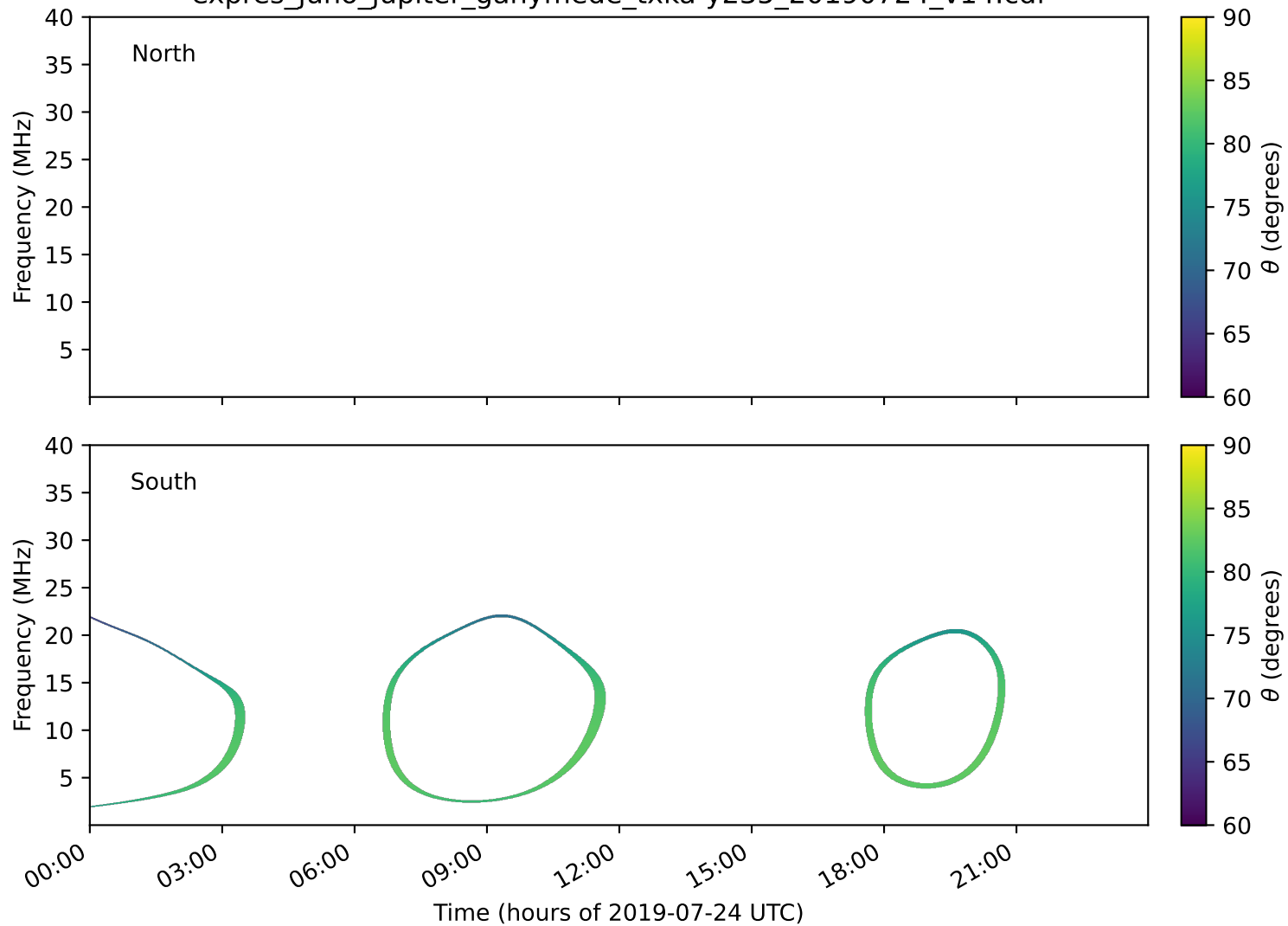
expres_juno_jupiter_ganymede_txka-y235_20190724_v14.cdf
