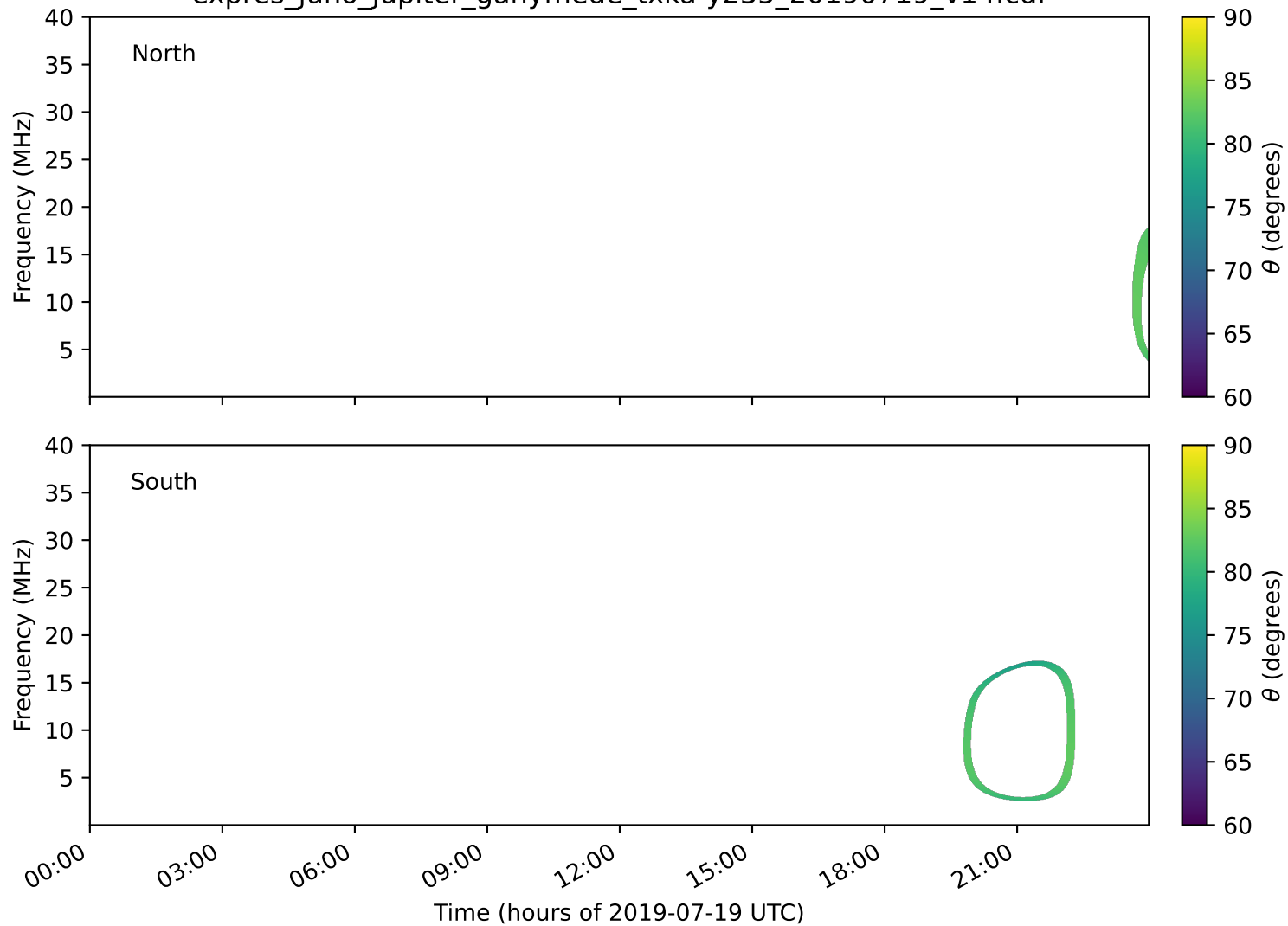
expres_juno_jupiter_ganymede_txka-y235_20190719_v14.cdf
