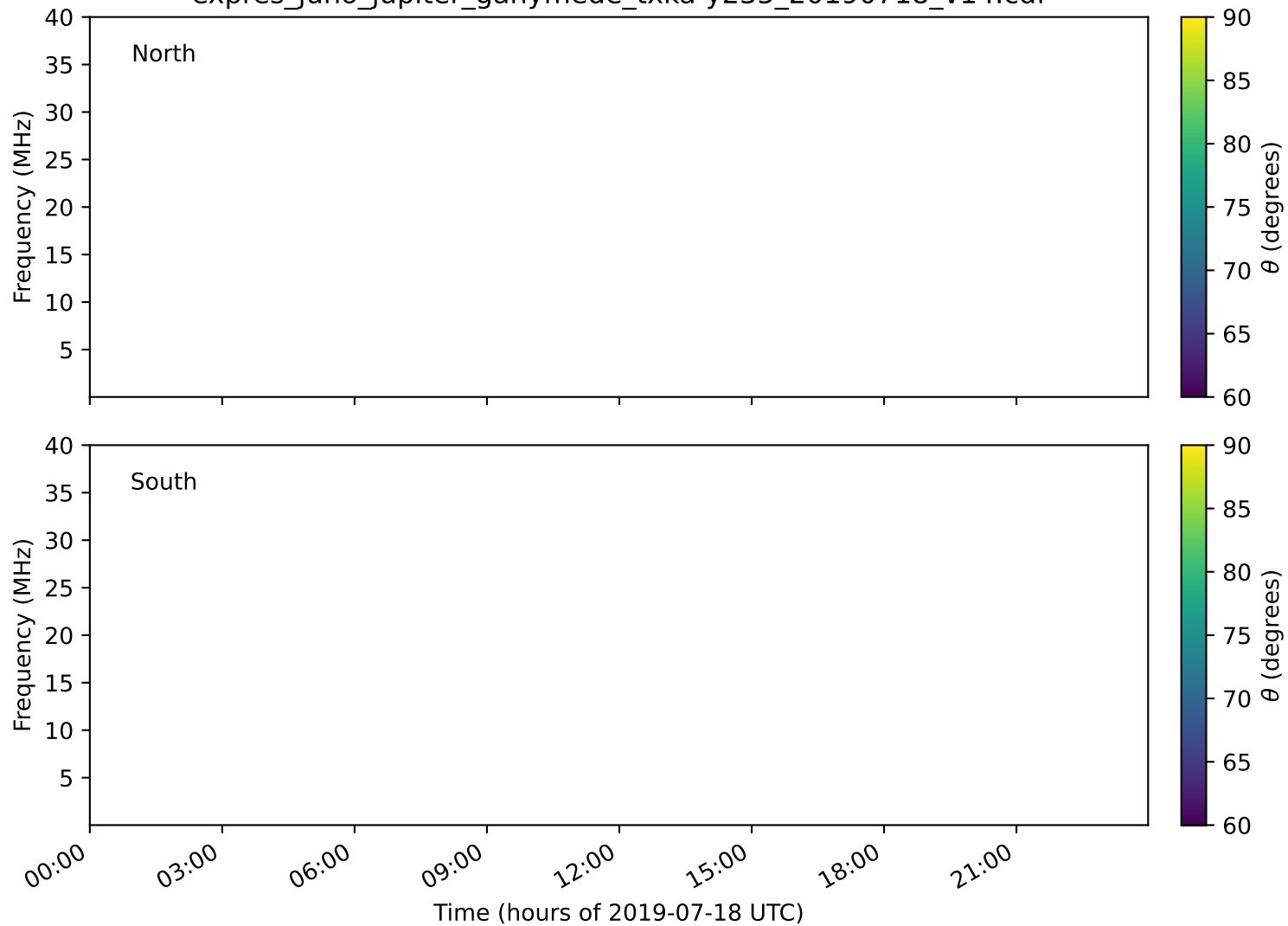
expres_juno_jupiter_ganymede_txka-y235_20190718_v14.cdf
