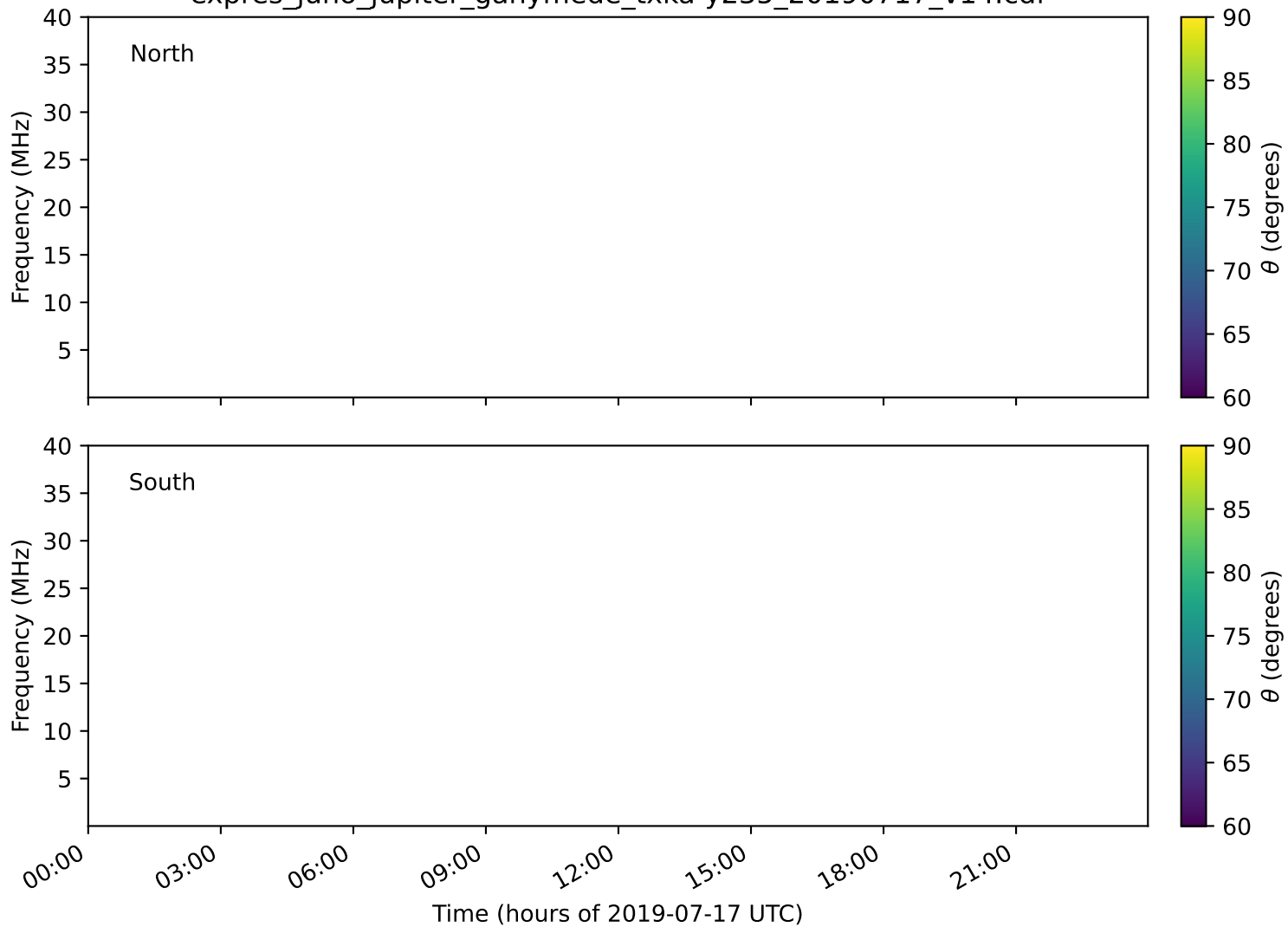
expres_juno_jupiter_ganymede_txka-y235_20190717_v14.cdf
