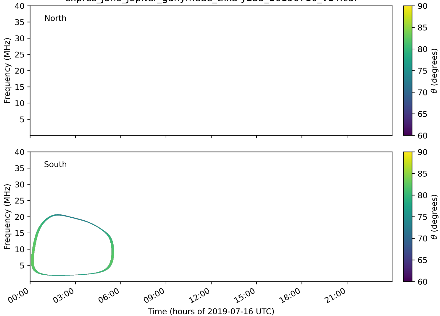
expres_juno_jupiter_ganymede_txka-y235_20190716_v14.cdf
