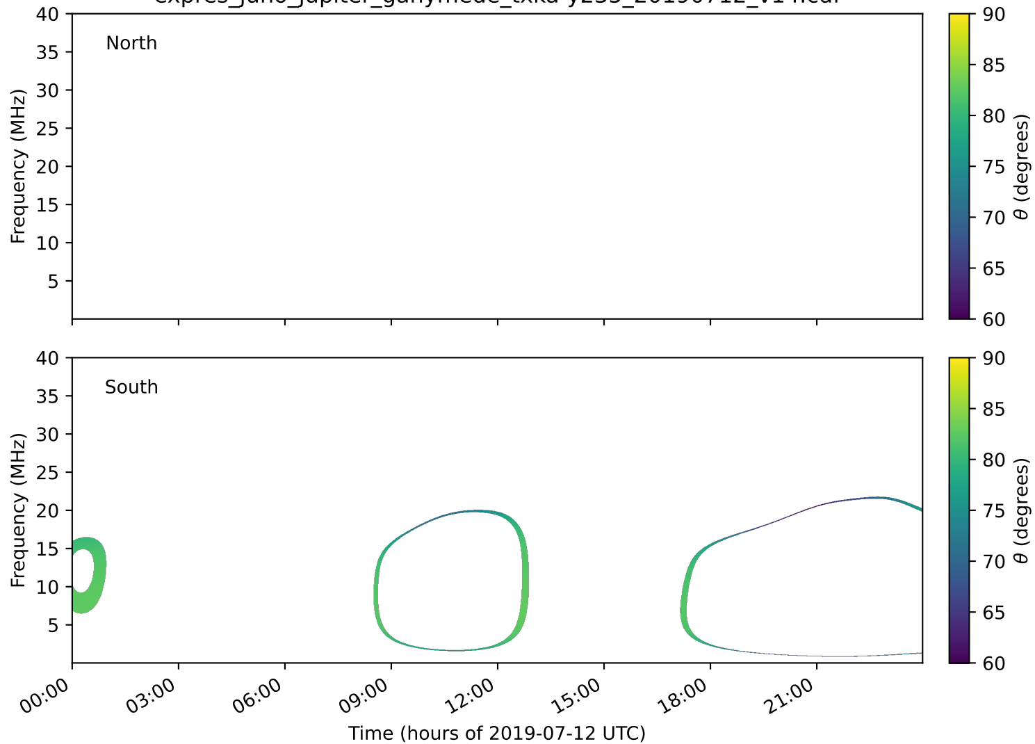
expres_juno_jupiter_ganymede_txka-y235_20190712_v14.cdf
