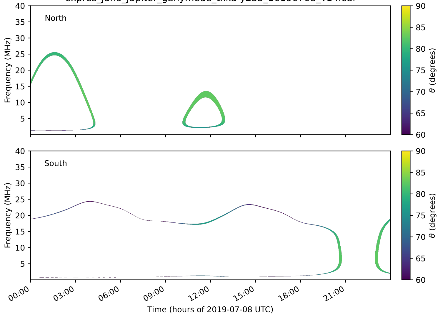
expres_juno_jupiter_ganymede_txka-y235_20190708_v14.cdf
