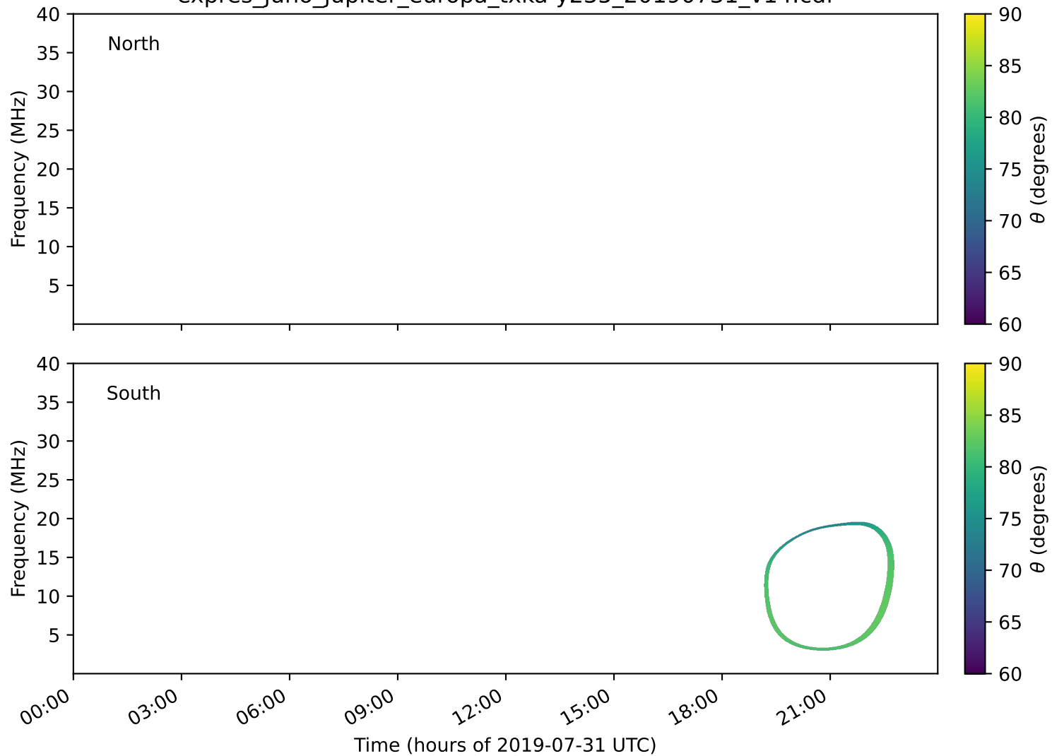
expres_juno_jupiter_europa_txka-y235_20190731_v14.cdf
