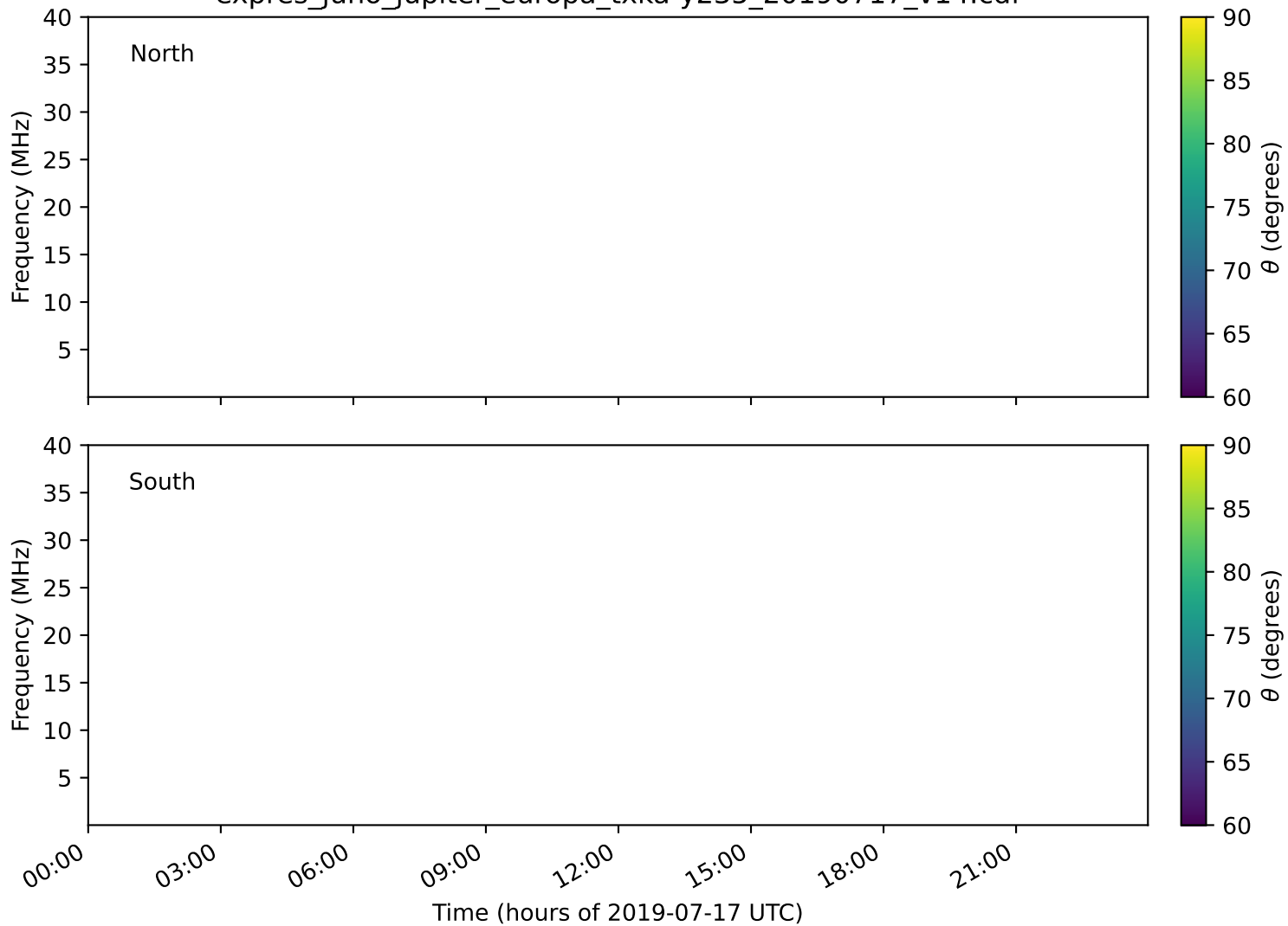
expres_juno_jupiter_europa_txka-y235_20190717_v14.cdf
