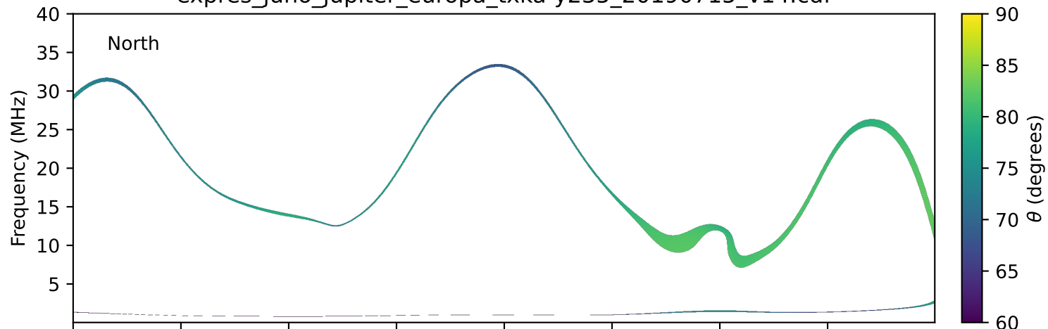
expres_juno_jupiter_europa_txka-y235_20190715_v14.cdf
