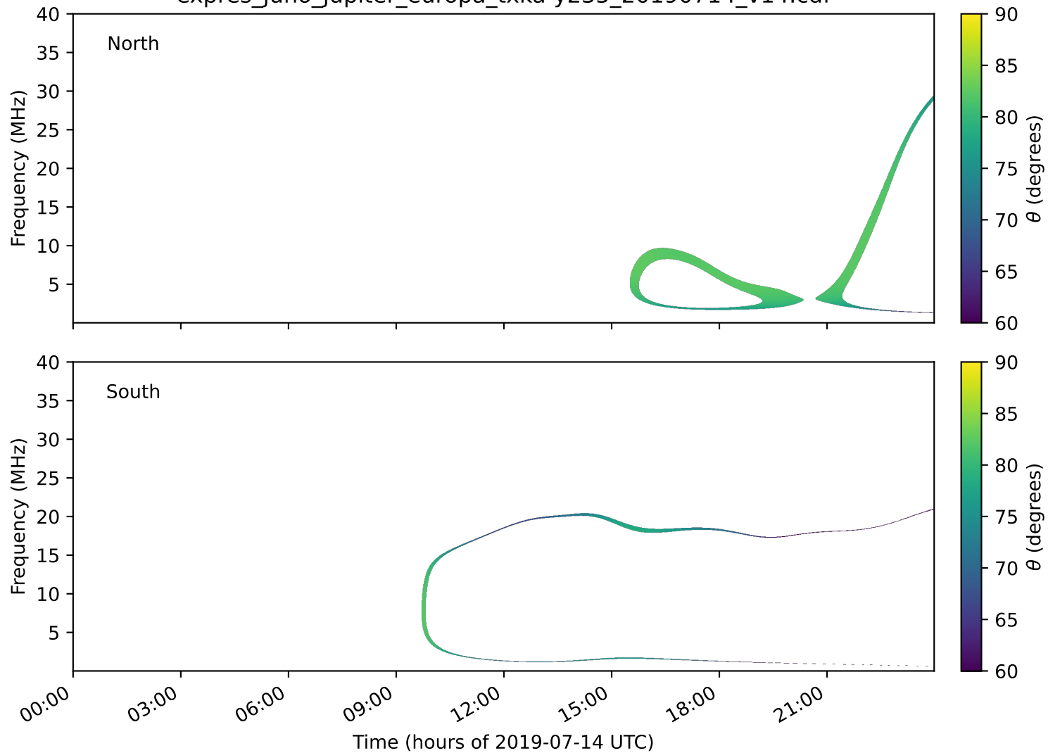
expres_juno_jupiter_europa_txka-y235_20190714_v14.cdf
