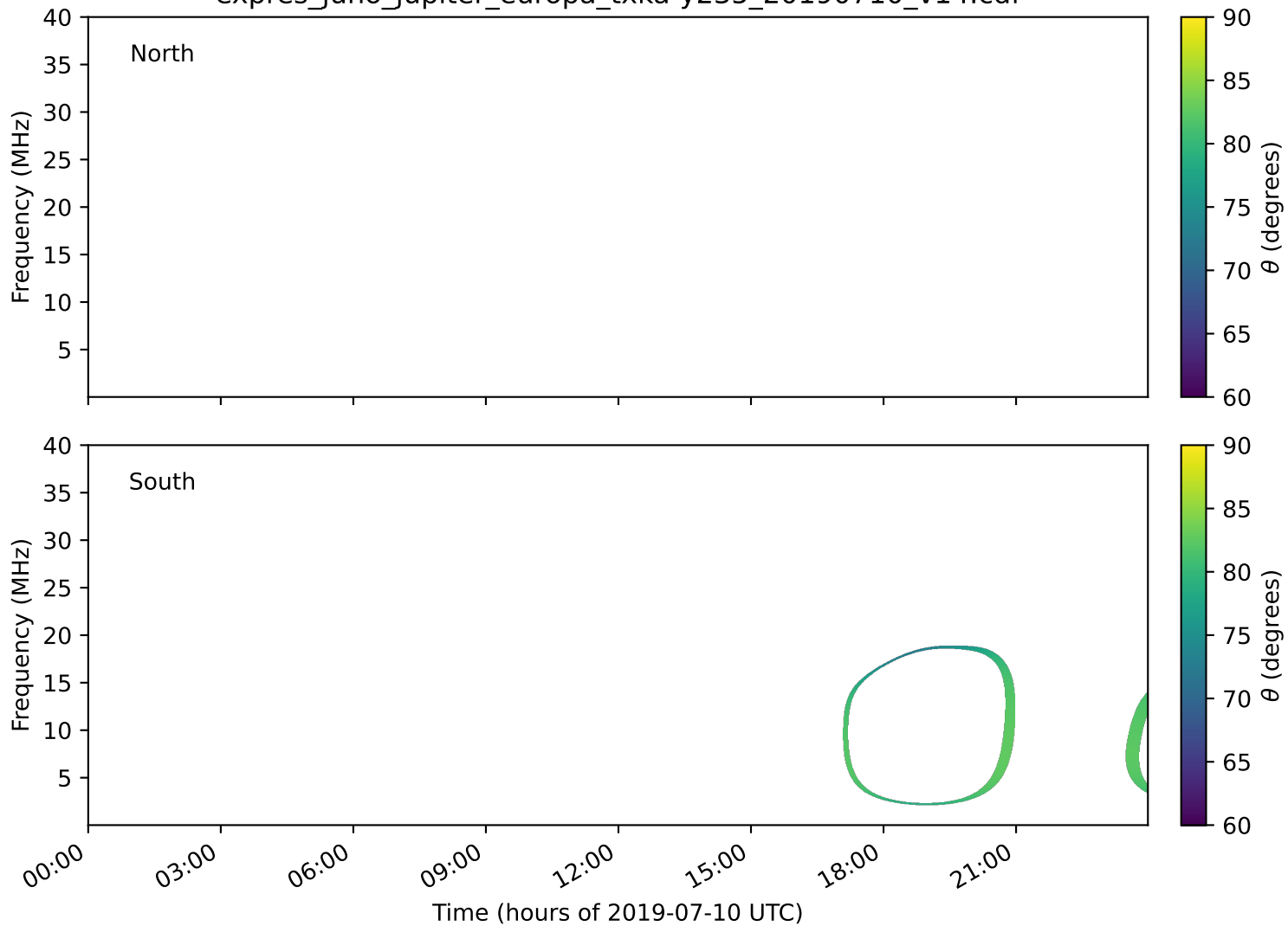
expres_juno_jupiter_europa_txka-y235_20190710_v14.cdf
