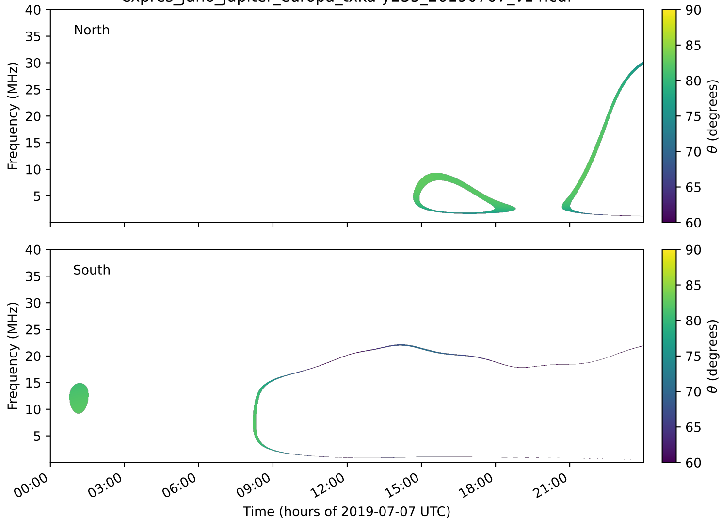
expres_juno_jupiter_europa_txka-y235_20190707_v14.cdf
