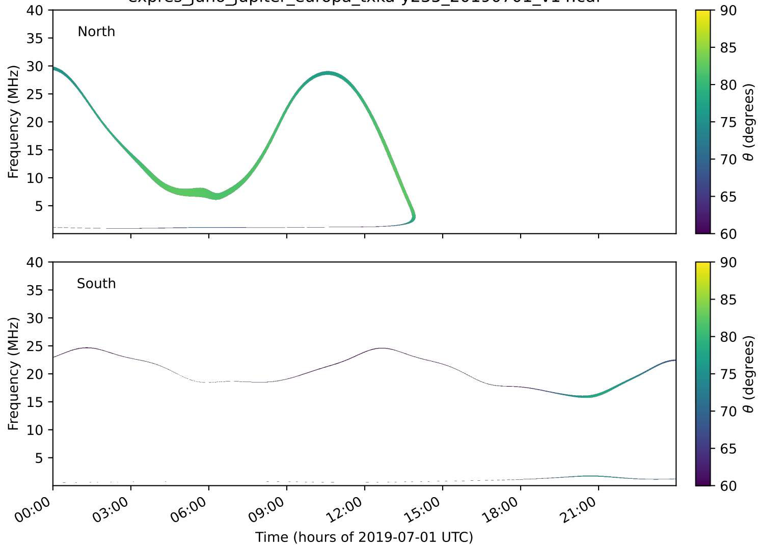
expres_juno_jupiter_europa_txka-y235_20190701_v14.cdf
