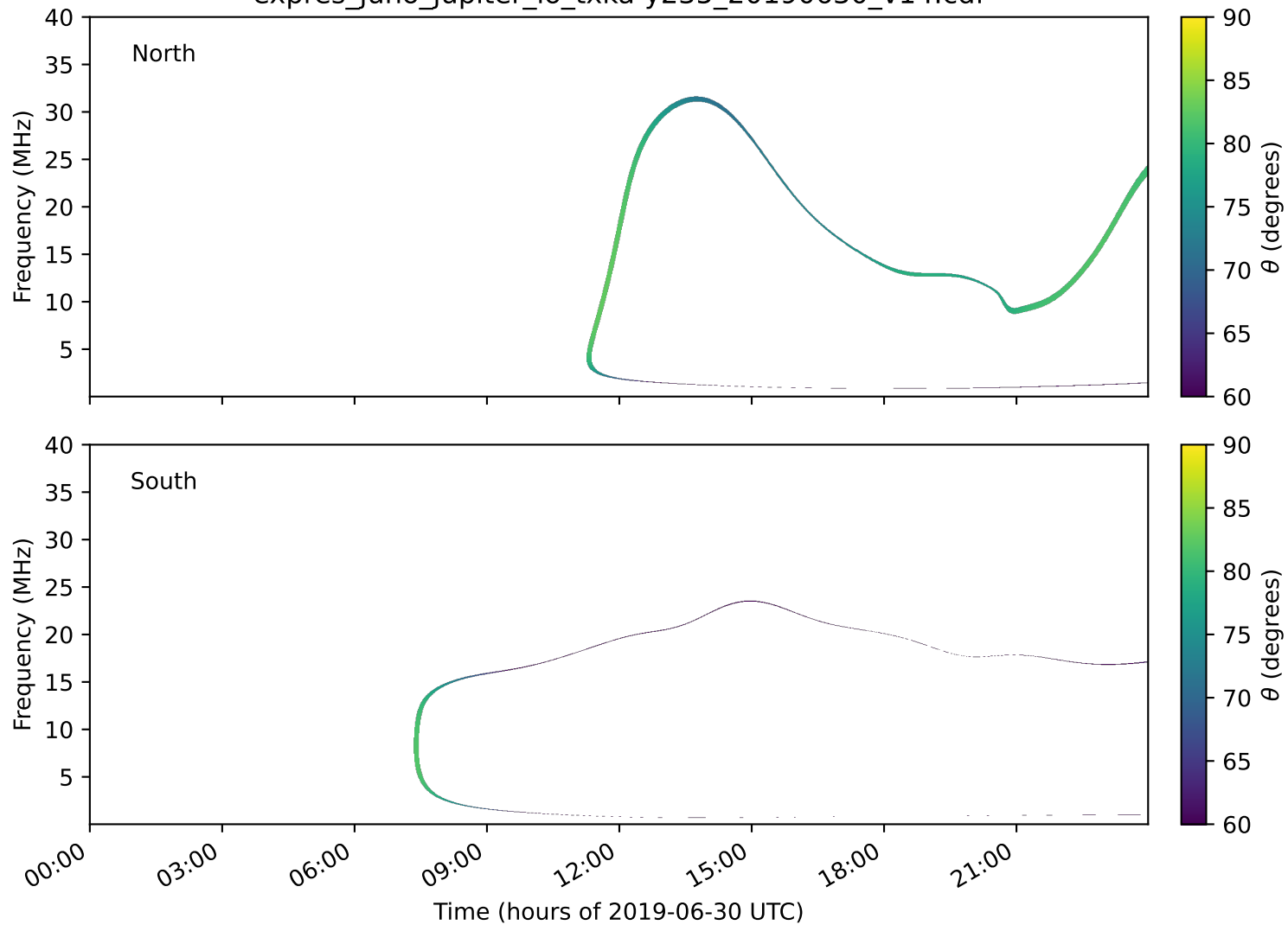
expres_juno_jupiter_io_txka-y235_20190630_v14.cdf
