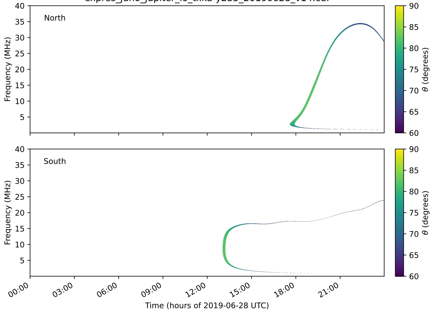
expres_juno_jupiter_io_txka-y235_20190628_v14.cdf
