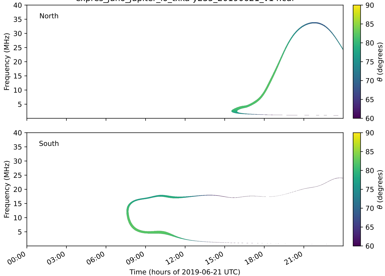
expres_juno_jupiter_io_txka-y235_20190621_v14.cdf
