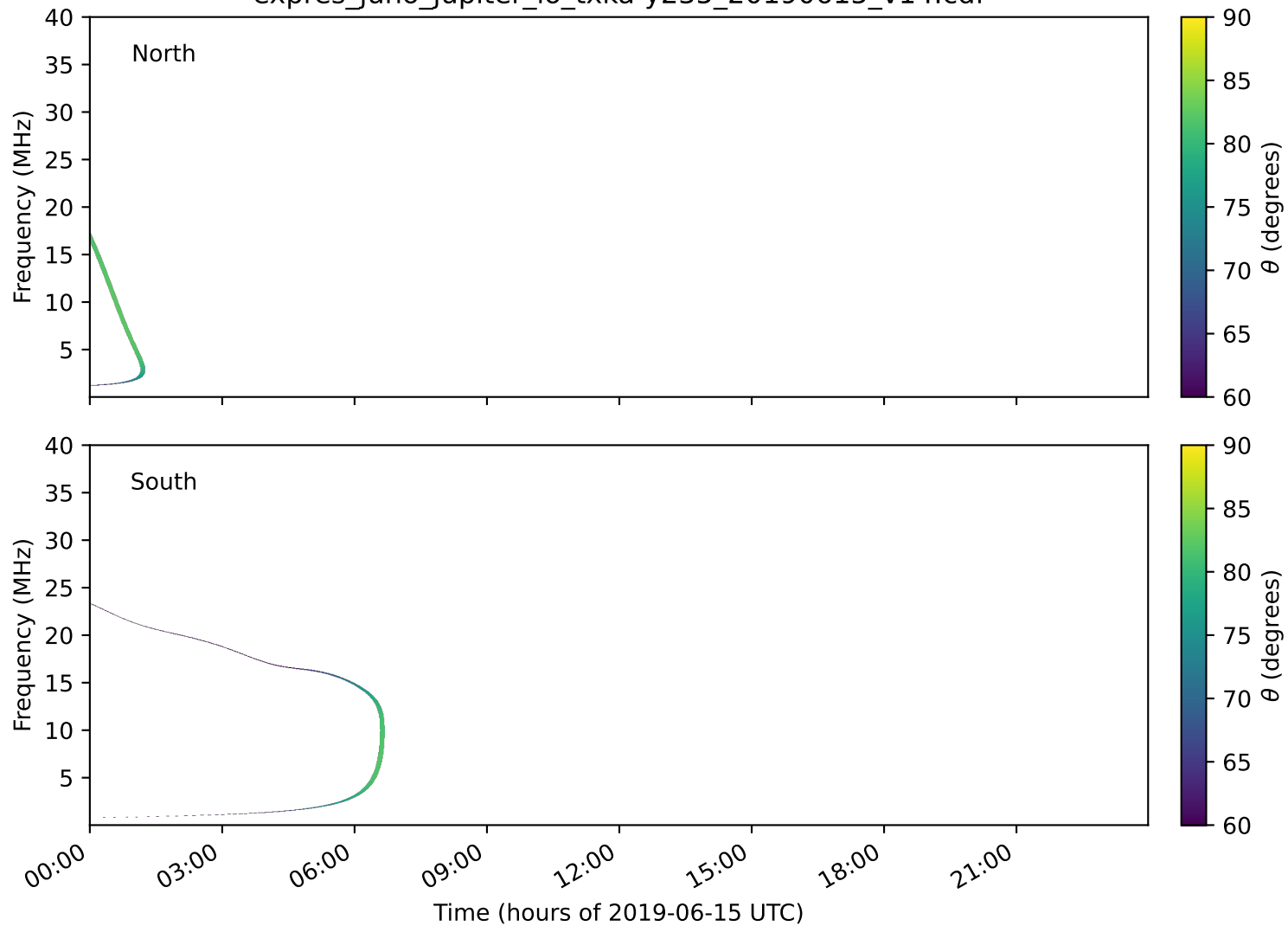
expres_juno_jupiter_io_txka-y235_20190615_v14.cdf
