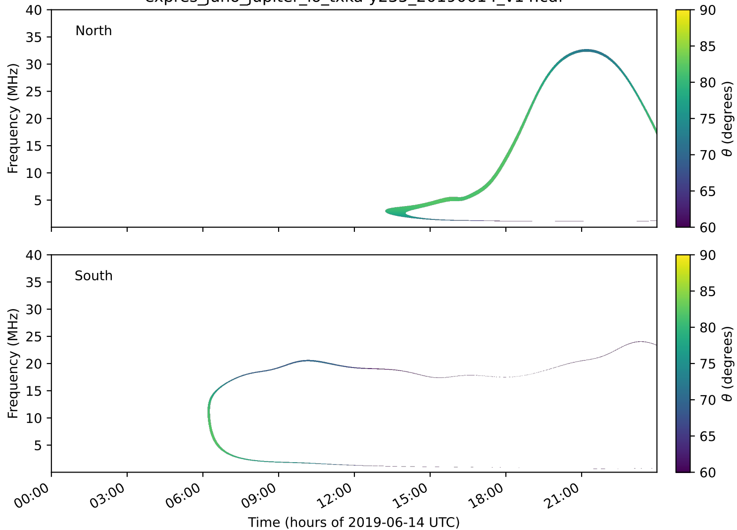
expres_juno_jupiter_io_txka-y235_20190614_v14.cdf
