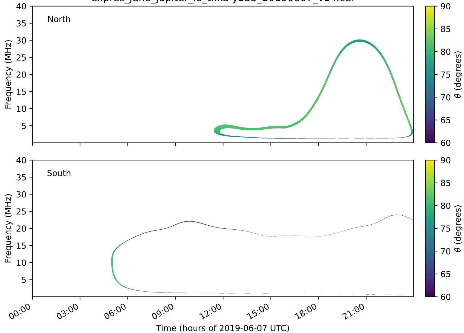
expres_juno_jupiter_io_txka-y235_20190607_v14.cdf
