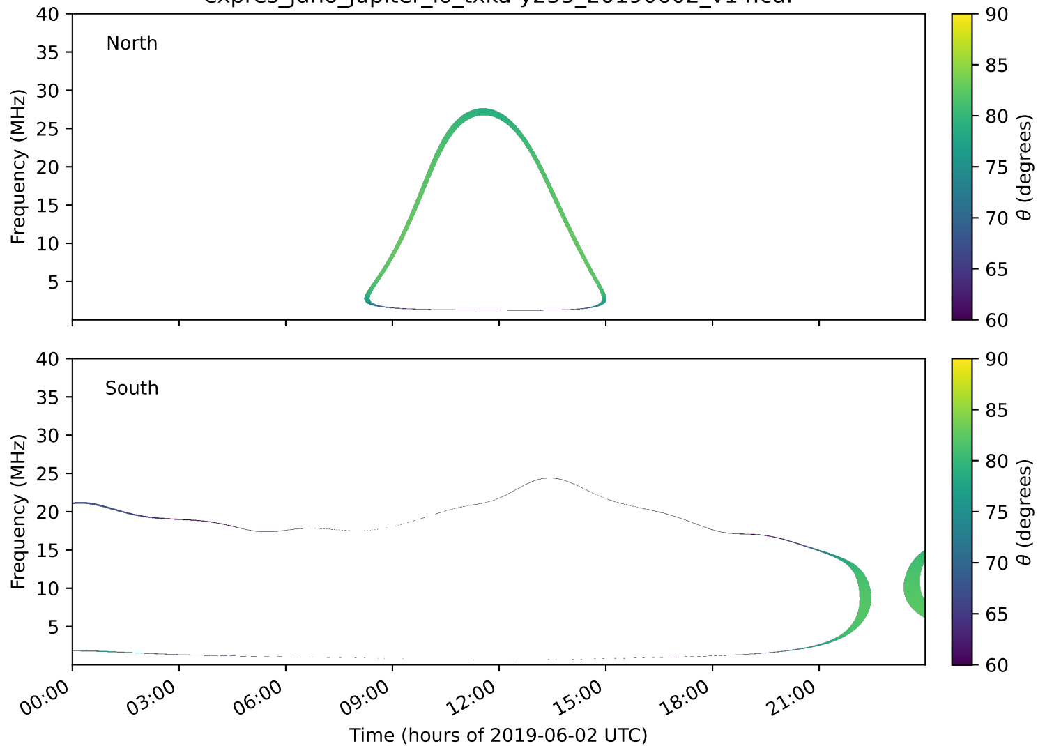
expres_juno_jupiter_io_txka-y235_20190602_v14.cdf
