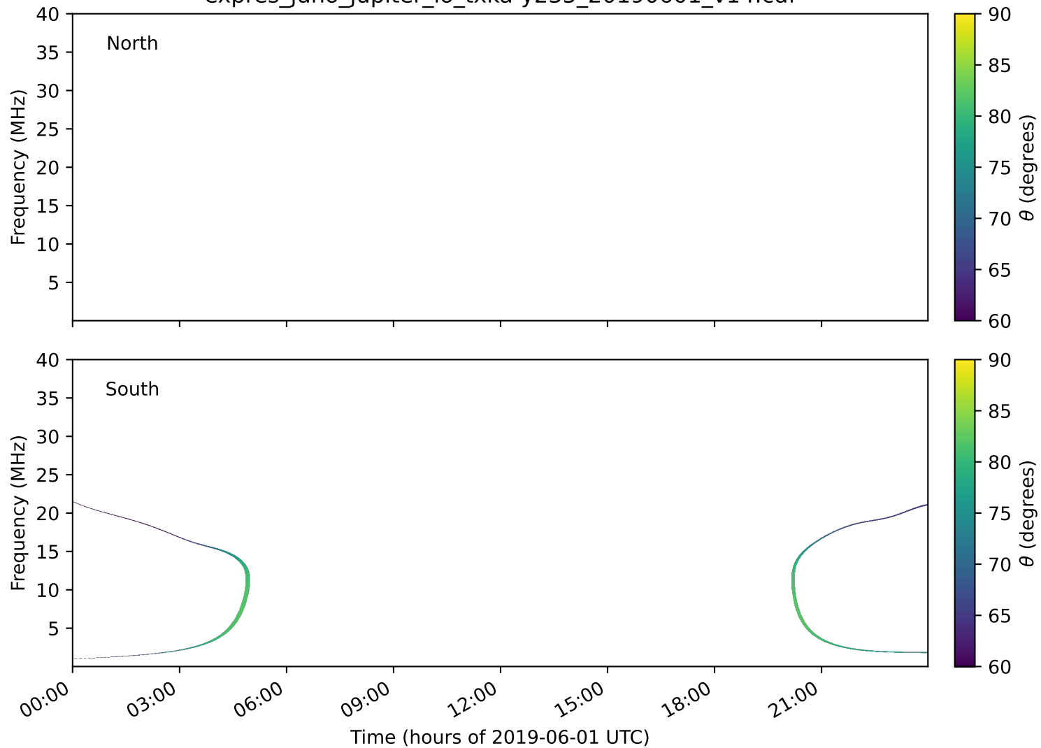
expres_juno_jupiter_io_txka-y235_20190601_v14.cdf
