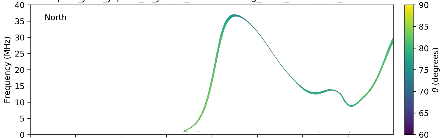
expres_juno_jupiter_io_jrm09_lossc-wid1deg_3kev_20190630_v01.cdf
