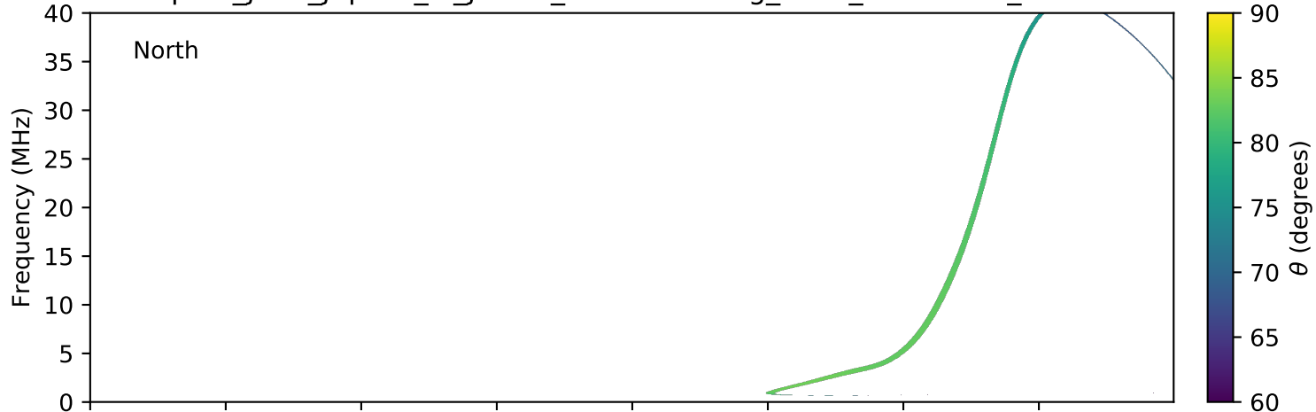
expres_juno_jupiter_io_jrm09_lossc-wid1deg_3kev_20190628_v01.cdf
