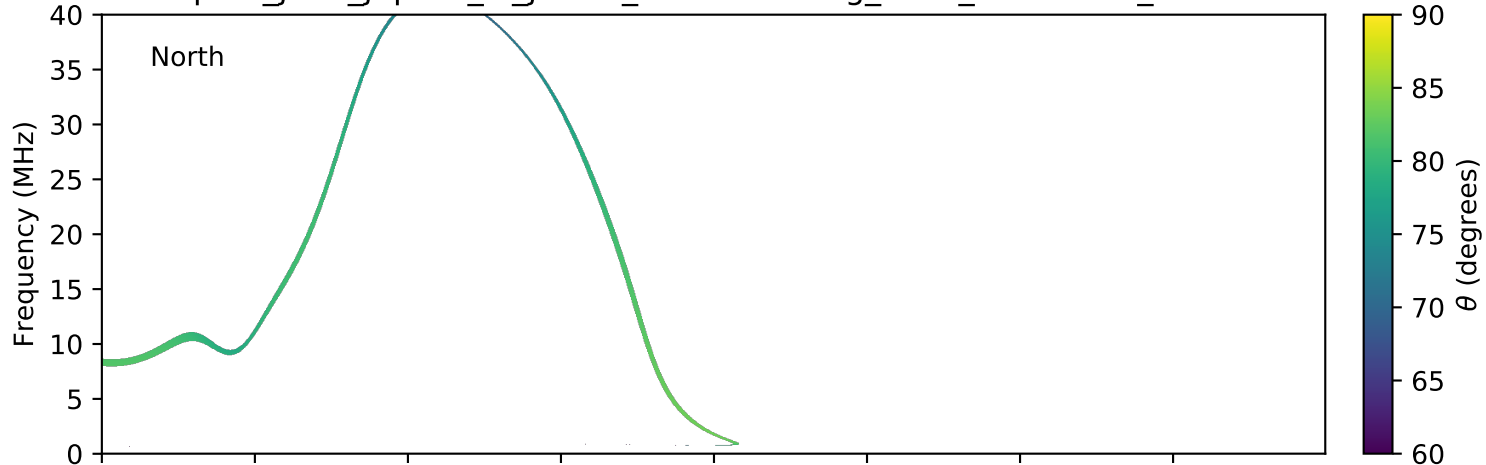
expres_juno_jupiter_io_jrm09_lossc-wid1deg_3kev_20190627_v01.cdf
